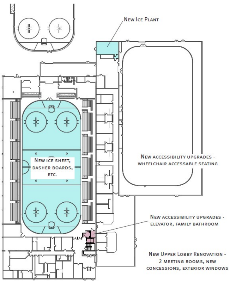
OVERALL LEVEL 1 FLOOR PLAN
